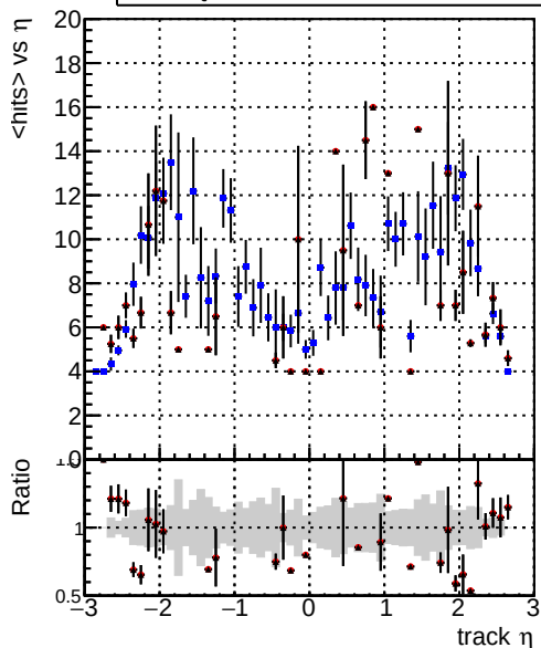
mean hit — DQM_CKF_TTbar — DQM_mkFit_TTbar — DQM_mkFit_TTbar-newTr2
