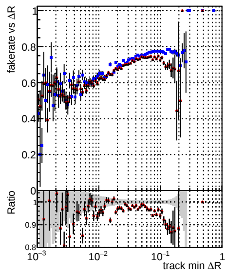
Legend: \blacksquare DQM_CKF_TTbar \bullet DQM_mkFit_TTbar \blacktriangleright DQM_mkFit_TTbar-newTr2
