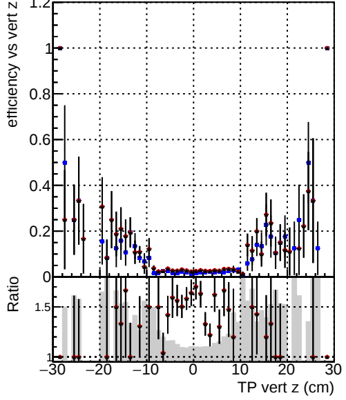
Efficiency vs. TP vert z (cm) — DQM_CKF_TTbar — DQM_mkFit_TTbar — DQM_mkFit_TTbar-newTr2
