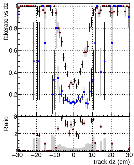
Fake rate vs dz — DOM CKF T\bar{T} bar — DOM mktFit T\bar{T} bar-newTr2
