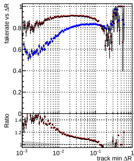
Legend: DQM_CKF_TTbar (blue circles) DQM_mkFit_TTbar (red circles) DQM_mkFit_TTbar-newTr2 (black circles) Fake rate vs \Delta R(\text{track, jet})
