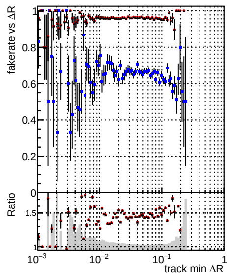
—●— DQM_CKF_TTbar —●— DQM_mkFit_TTbar —●— DQM_mkFit_TTbar-newTr2
