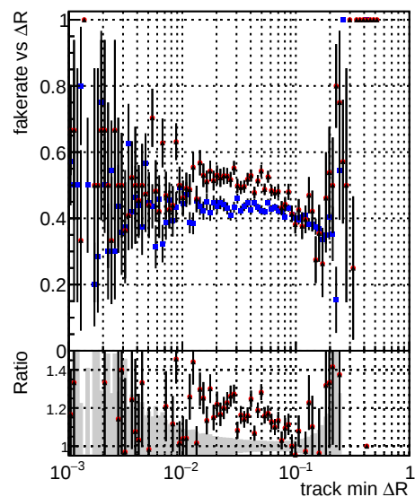
Legend: DQM_CKF_TTbar (blue squares) DQM_mkFit_TTbar (red circles) DQM_mkFit_TTbar-newTr2 (black triangles) Fake rate vs \Delta R(\text{track, jet})
