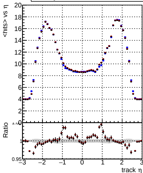
mean hit — DQM_CKF_TTbar — DQM_mkFit_TTbar — DQM_mkFit_TTbar-newTr2
