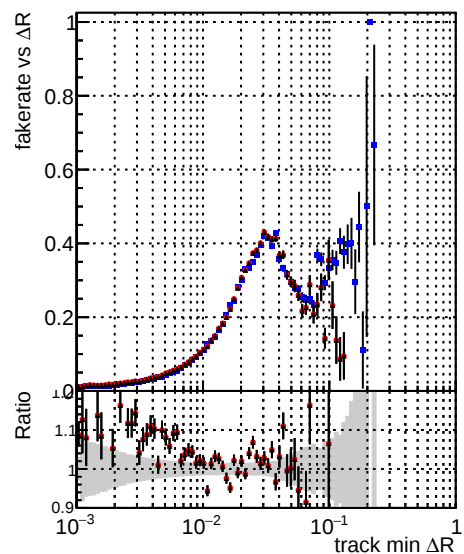
Legend for Fake rate vs \Delta R , Duplicates Rate vs \Delta R , and Pileup rate vs \Delta R : \blacksquare DOM_CKF_TTbar \bullet DOM_mkFit_TTbar \blacktriangledown DOM_mkFit_TTbar-newTr
