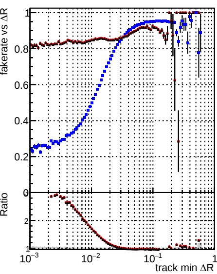
Fake rate vs \Delta R(\text{track, jet}) Legend: DOM_CKF_TTbar (blue line with dots) DOM_mkFit_TTbar (red line with dots) DOM_mkFit_TTbar-newTr (black line with dots)
