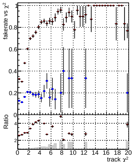
Fake rate vs. DOM CKF TTbar DOM mkFit TTbar-newTr
