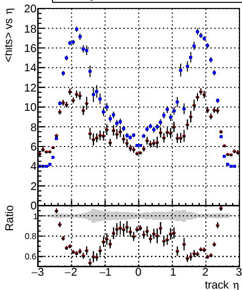
mean hit — DQM_CKF_TTbar — DQM_mkFit_TTbar — DQM_mkFit_TTbar-newTr
