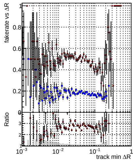
—●— DQM_CKF_TTbar —●— DQM_mkFit_TTbar —●— DQM_mkFit_TTbar-newTr
