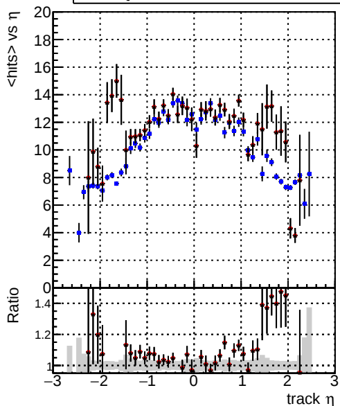
mean hit — DQM_CKF_TTbar — DQM_mkFit_TTbar — DQM_mkFit_TTbar-newTr
