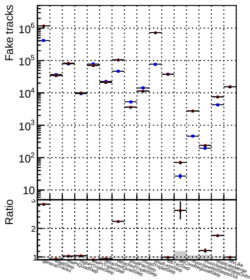
Number DQM_CKF_TTbar DQM_mkFit_TTbarPU-ncp DQM_mkFit_TTbarPU-newTr6
