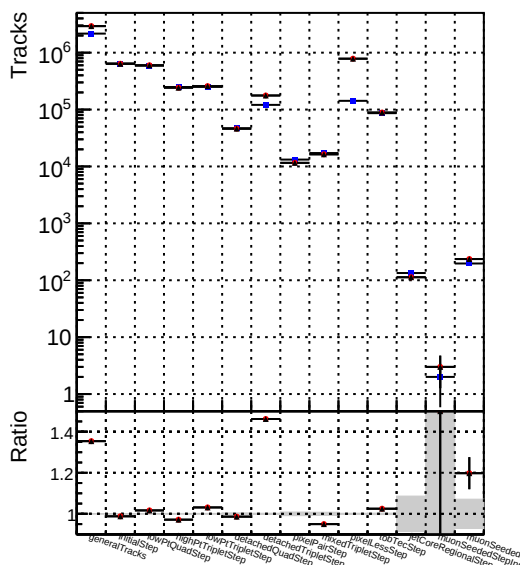
—●— DQM_CKF_TTbar —●— DQM_mkFit_TTbarPU-ncp —●— DQM_mkFit_TTbarPU-newTr6
