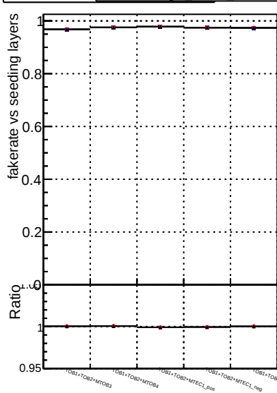
Fake rate vs. DOM CKF TTbar BOM mktT TTbarPU-nep BOM mktT TTbarPU-newTr6
