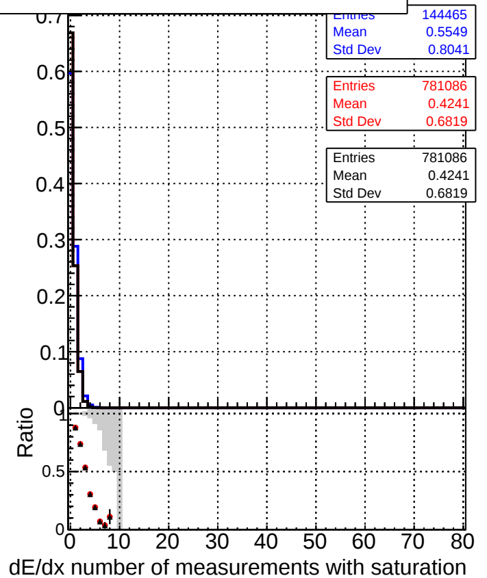
DQM_CKF_TTbar DQM_mkFit_TTbarPU-ncp DQM_mkFit_TTbarPU-newTr6
