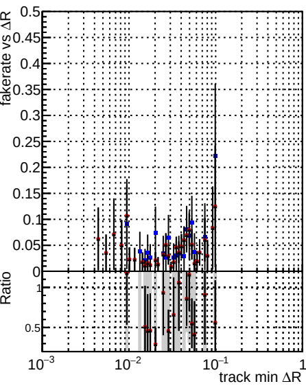
Fake rate vs \Delta R(\text{track}, \text{jet}) DOM_CKF_TTbar DOM_mkFit_TTbarPU-ncp DOM_mkFit_TTbarPU-newTr6
