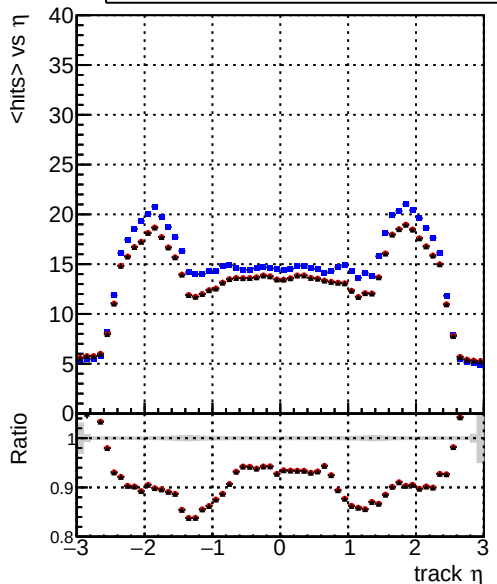
mean hit — DQM_CKF_TTbar — DQM_mkFit_TTbarPU-ncp — DQM_mkFit_TTbarPU-newTr6
