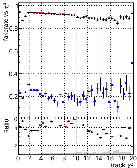
Fake rate vs. DOM CKE TTbar DOM mkttt TTbarPU-ncp DOM mkttt TTbarPU-newTr6
