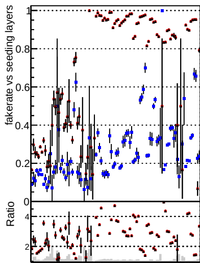
Fake rate vs. DOM CKE TTbar DOM mkttt TTbarPU-ncp DOM mkttt TTbarPU-newTr6
