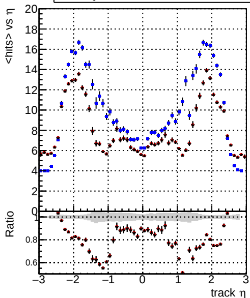
mean hits — DQM_CKF_TTbar — DQM_mkFit_TTbarPU-ncp — DQM_mkFit_TTbarPU-newTr6
