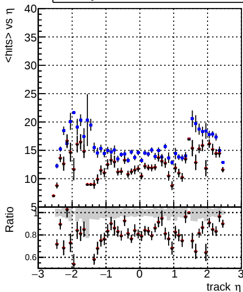
mean hits vs \eta — DQM_CKF_TTbar — DQM_mkFit_TTbarPU-ncp — DQM_mkFit_TTbarPU-newTr6
