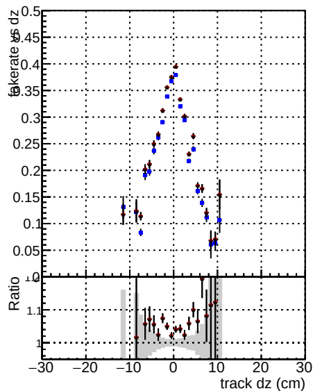
— DOM CKE TTbar — DOM mktFit TTbarPU-ncp — DOM mktFit TTbarPU-newTr6
