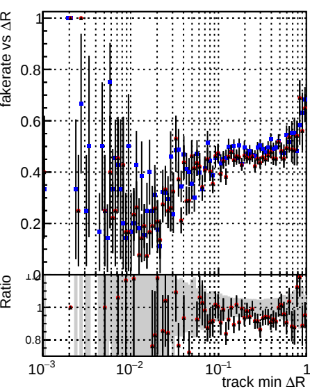
Legend: DQM_CKF_TTbar (blue circles), DQM_mkFit_TTbarPU-ncp (red circles), DQM_mkFit_TTbarPU-newTr6 (black circles)
