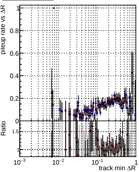
Legend: DOM_CKF_TTbar (blue circles), DOM_mkFit_TTbarPU-ncp (red circles), DOM_mkFit_TTbarPU-newTr6 (black circles)
