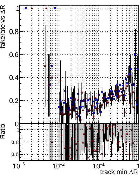
Legend: DOM_CKF_TTbar (blue circles), DOM_mkFit_TTbarPU-ncp (red circles), DOM_mkFit_TTbarPU-newTr6 (black circles)
