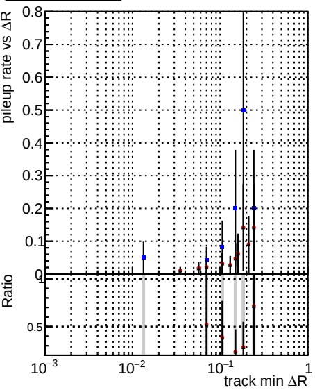
DOM_CKF_TTbar DOM_mkFit_TTbarPU-ncp DOM_mkFit_TTbarPU-newTr6
