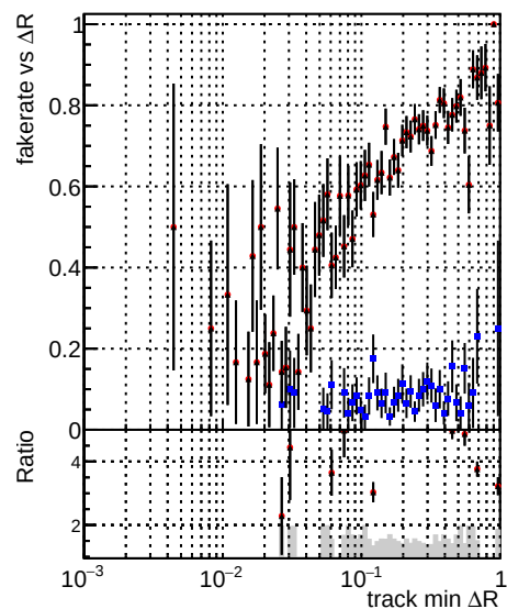
Legend: DQM_CKF_TTbar (black circles) DQM_mkFit_TTbarPU-ncp (red circles) DQM_mkFit_TTbarPU-newTr6 (blue circles)
