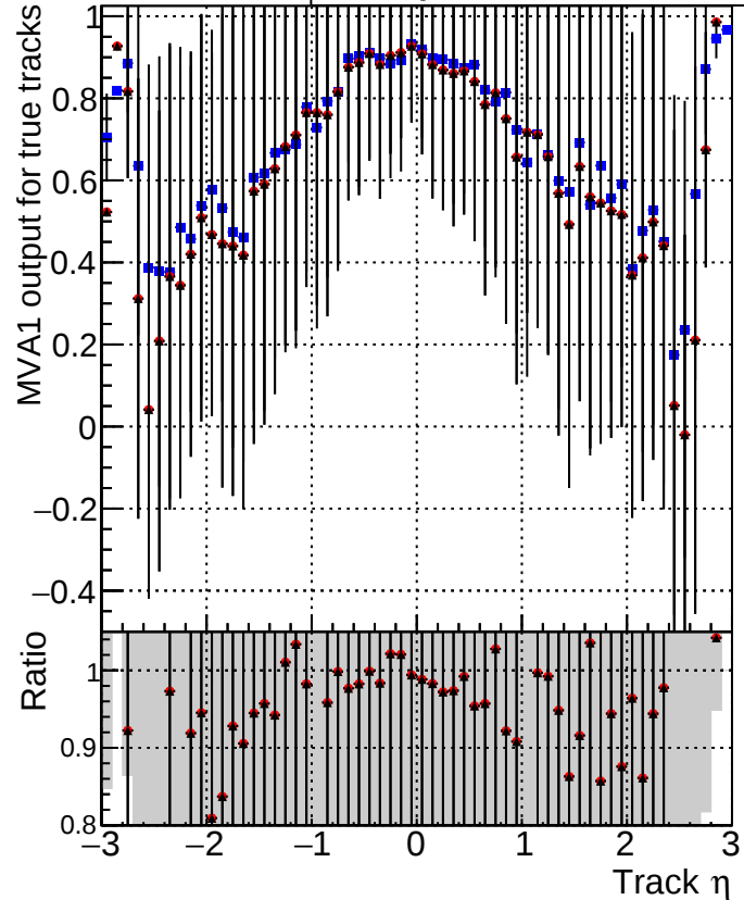
MVA1 of associated tracks (recoToSim) vs. track \eta Legend: DQM_CKF_TTbar (blue squares) DQM_mkFit_TTbarPU-ncp (red circles) DQM_mkFit_TTbarPU-newTr6 (black triangles)
