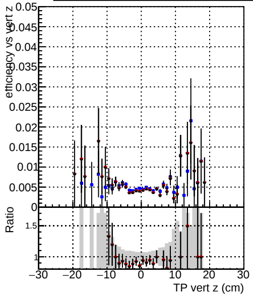
Efficiency vs vert z — DQM_CKF_TTbar — DQM_mkFit_TTbarPU-ncp — DQM_mkFit_TTbarPU-newTr6
