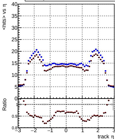
mean hit — DQM_CKF_TTbar — DQM_mkFit_TTbarPU-ncp — DQM_mkFit_TTbarPU-newTr6
