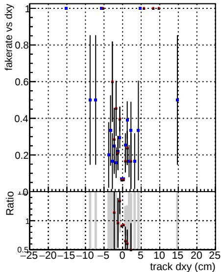
Legend for Fake rate vs d, Duplicates Rate vs Dxy, and Pileup rate vs dxy plots: DOM CKF T\bar{T} bar DOM CKF T\bar{T} barPU-ncp DOM CKF T\bar{T} barPU-newTr6
