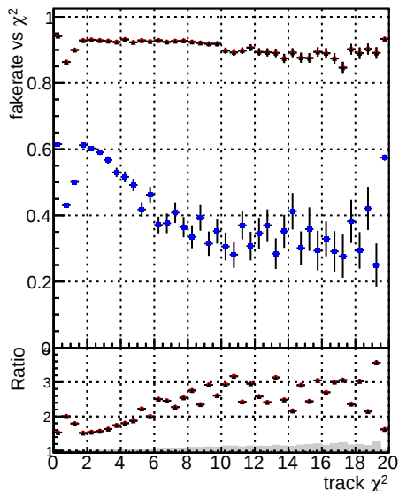
Fake rate vs. DOM CKF TTbar DOM mktFit TTbarPU-ncp DOM mktFit TTbarPU-newTr6
