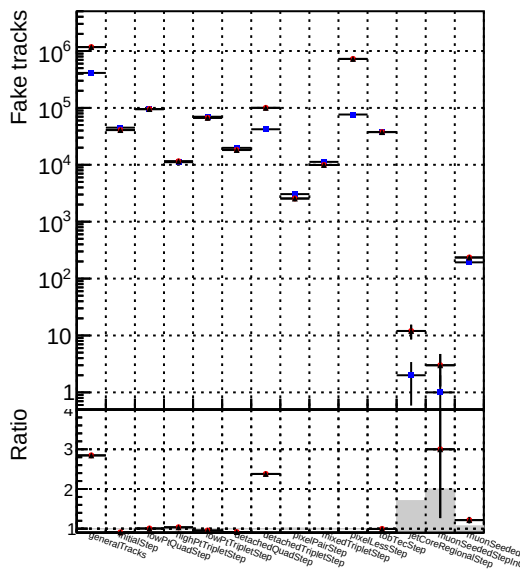
Number of tracks DQM_CKF_TTbar DQM_mkFit_TTbarPU-ncp DQM_mkFit_TTbarPU-newTr5
