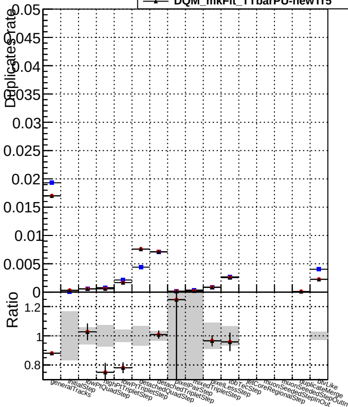
Duplicates rate vs \epsilon —●— DQM_mkFit_TTbarPU-ncp —▲— DQM_mkFit_TTbarPU-newTr5
