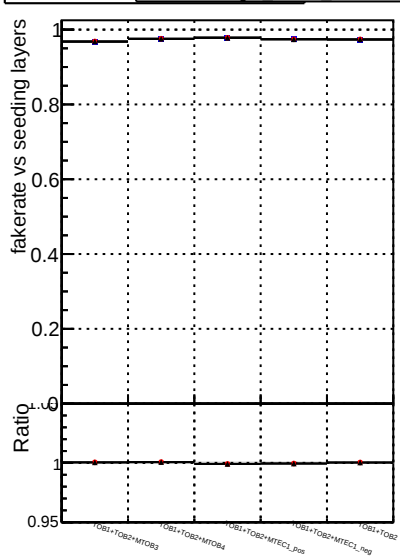
Fake rate vs. Legend: DOM CKF TTbar DOM CKF TTbarPU-ncp DOM CKF TTbarPU-newTr5
