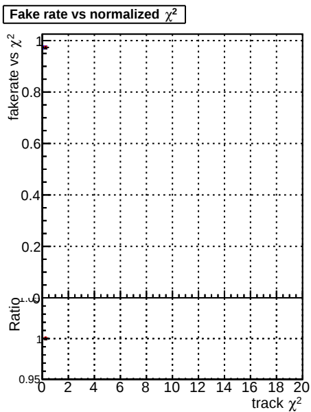
Fake rate vs. Legend: DOM CKF TTbar DOM CKF TTbarPU-ncp DOM CKF TTbarPU-newTr5
