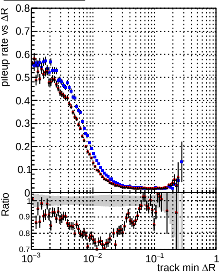
Legend: —•— DQM_CKF_TTbar —•— DQM_mkFit_TTbarPU-ncp —•— DQM_mkFit_TTbarPU-newTr5
