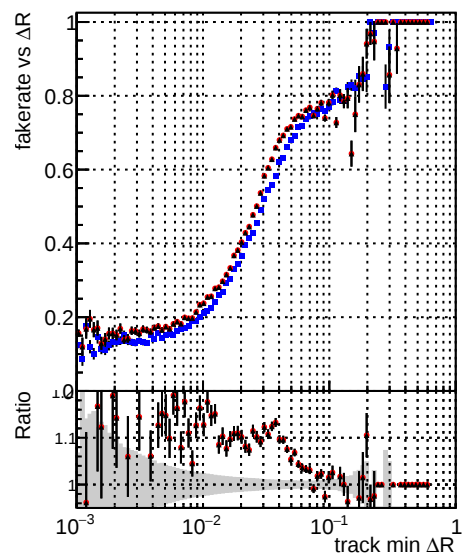
Legend: \blacksquare DOM_CKF_TTbar \bullet DOM_mkFit_TTbarPU-ncp \blacktriangleright DOM_mkFit_TTbarPU-newTr5
