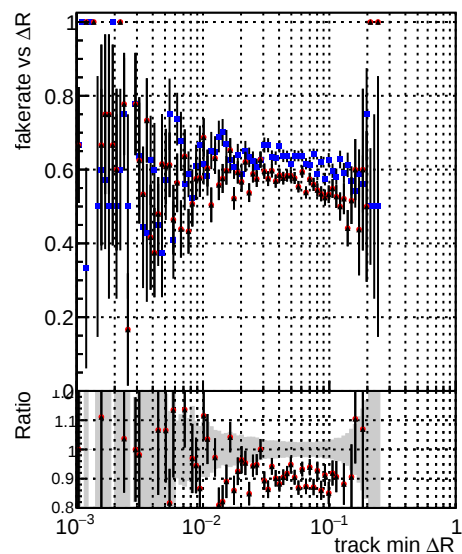
—●— DQM_CKF_TTbar —●— DQM_mkFit_TTbarPU-ncp —●— DQM_mkFit_TTbarPU-newTr5
