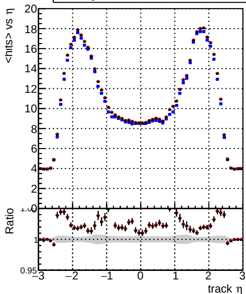
mean hits DQM_CKF_TTbar DQM_mkFit_TTbarPU-ncp DQM_mkFit_TTbarPU-newTr5
