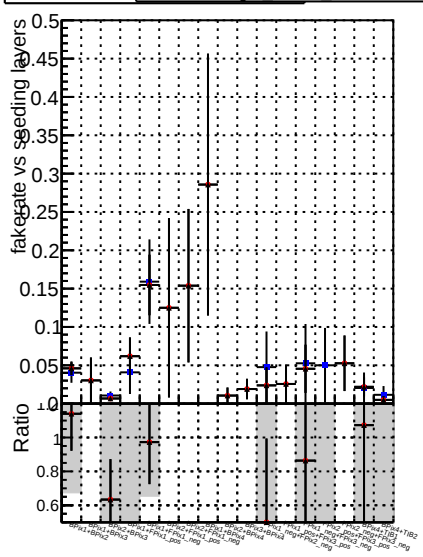
Fake rate vs. \bar{t}t t\bar{t} t\bar{t} + \text{bkg} t\bar{t} + \text{bkg} + \text{PU}
