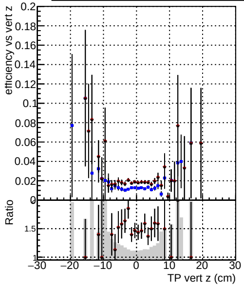
Efficiency vs vert z — DQM_CKF_TTbar — DQM_mkFit_TTbarPU-ncp — DQM_mkFit_TTbarPU-newTr5
