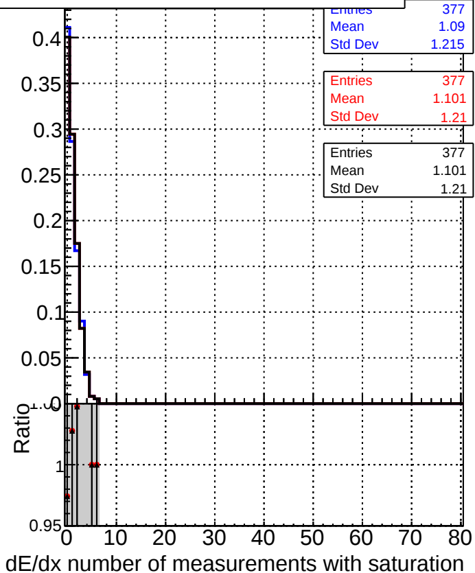
—■ DQM_CKF_TTbar —● DQM_mkFit_TTbarPU-ncp —● DQM_mkFit_TTbarPU-newTr5
