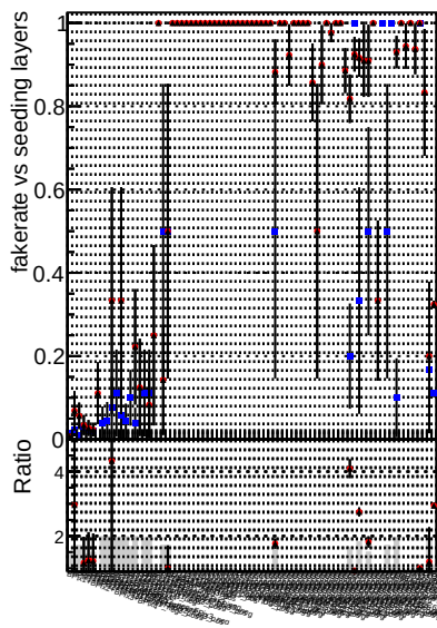
Fake rate vs. DOM CKF TTbar DOM CKF TTbar PU-nep DOM CKF TTbar PU-newTr5
