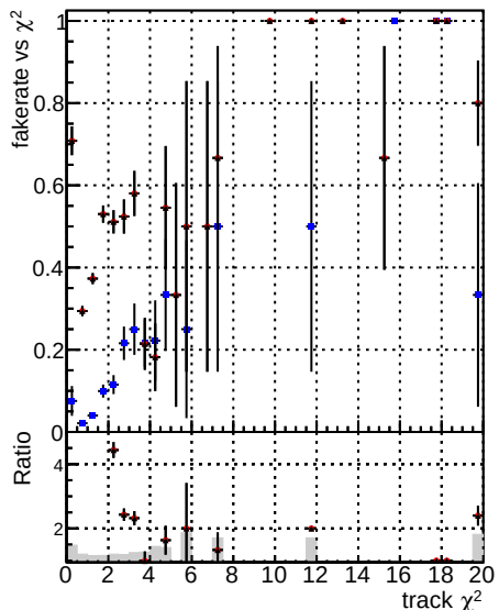
Fake rate vs. DOM CKF TTbar DOM CKF TTbar PU-nep DOM CKF TTbar PU-newTr5
