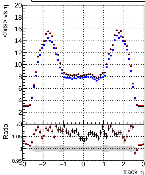
mean hits DQM_CKF_TTbar DQM_mkFit_TTbarPU-ncp DQM_mkFit_TTbarPU-newTr5
