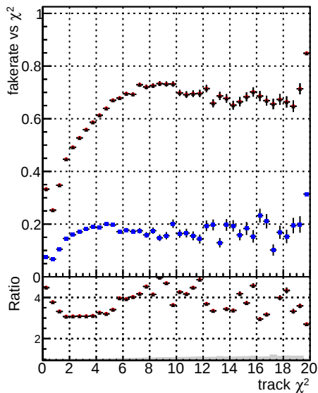
Fake rate vs. DOM CKF TTbar DOM mktT TTbarPU-nct DOM mktT TTbarPU-nctTr5
