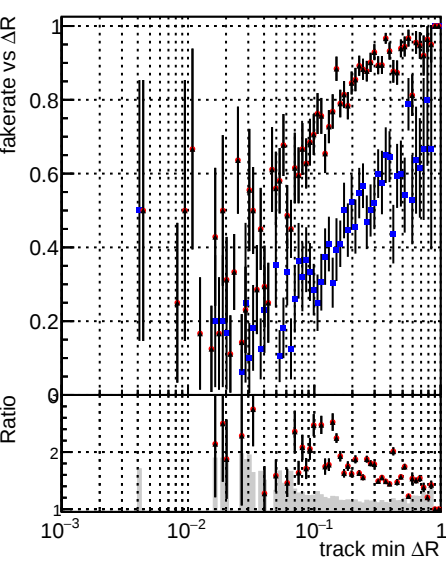
Fake rate vs \Delta R(\text{track, jet}) DQM_CKF_TTbar DQM_mkFit_TTbarPU-ncp DQM_mkFit_TTbarPU-newTr5
