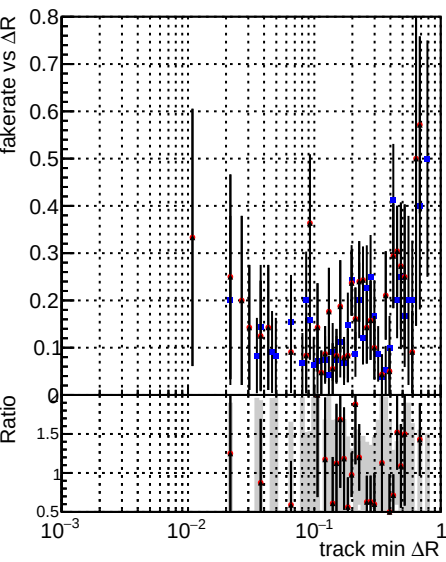
● DQM_CKF_TTbar ● DQM_mkFit_TTbarPU-ncp ● DQM_mkFit_TTbarPU-newTr5
