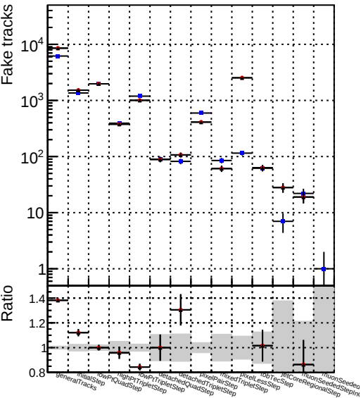
Number Legend ● DQM_mkFit_TTbarPU-hcp ▲ DQM_mkFit_TTbarPU-newTr5
