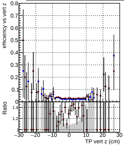
Efficiency vs. TP vert z (cm) — DQM_CKF_TTbar — DQM_mkFit_TTbarPU-ncp — DQM_mkFit_TTbarPU-newTr5
